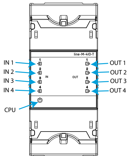
Figura 15: LEDs: line-M-4IO-T.
